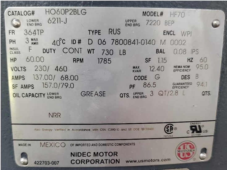
High Service Pump Motor Nameplate
