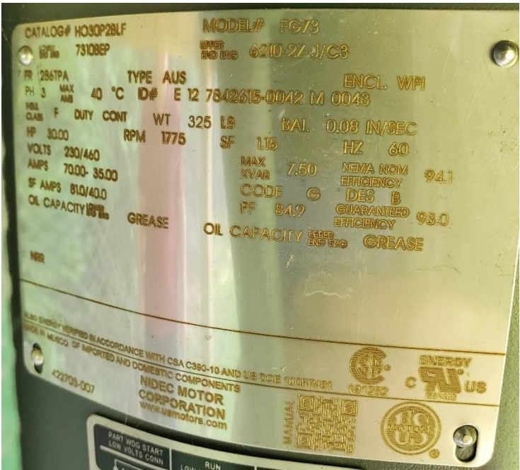
Well Pump Motor Nameplate
